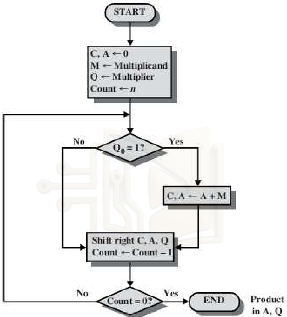
Fig. Flow chart of unsigned binary multiplication
