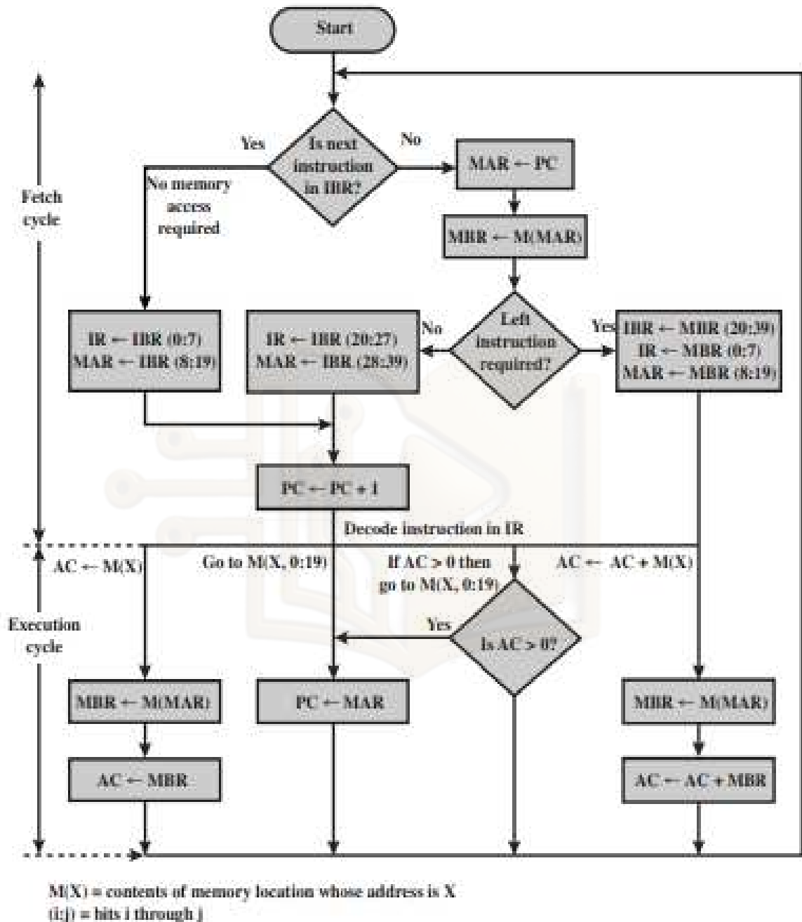
Figure 2.4 Partial Flowchart of IAS Operation
