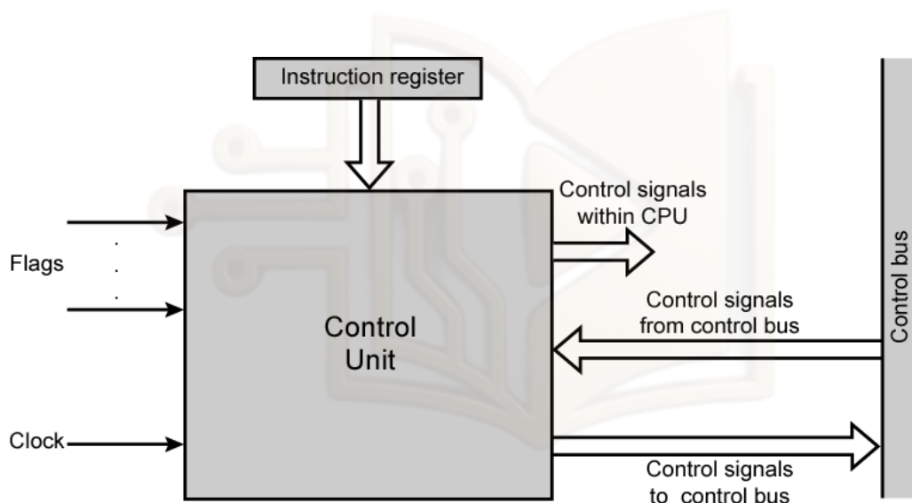
Fig. Block diagram of a control unit.
