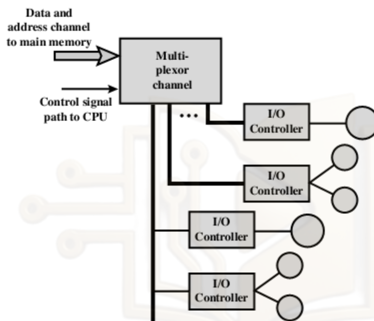
(b) Multiplexor
