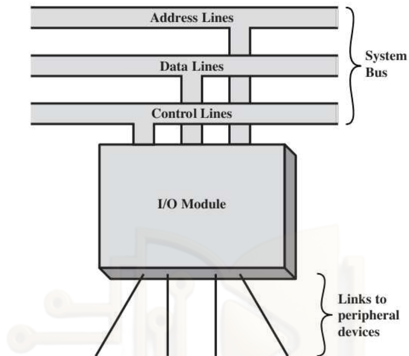
Fig: Generic model of I/O model
